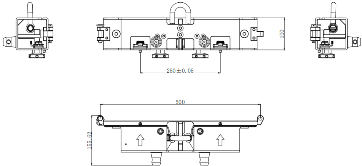
Iridah 500mm hanging and stacking beam
