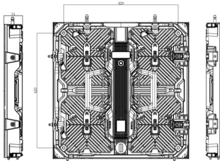
500×500mm Cabinet
