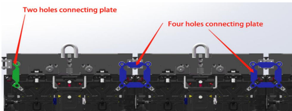
Fix connecting plate
