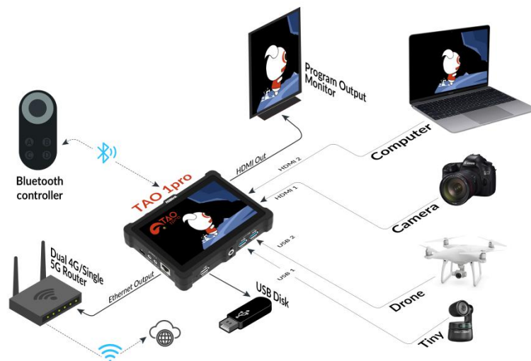
SYSTEM CONNECTION
