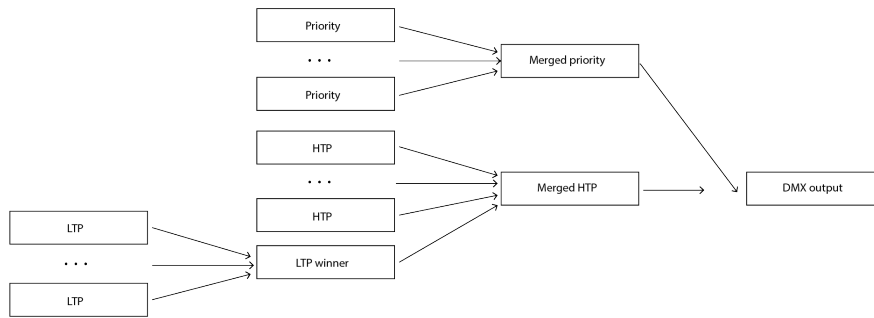
Figure 10.3: DMX merging precedence
