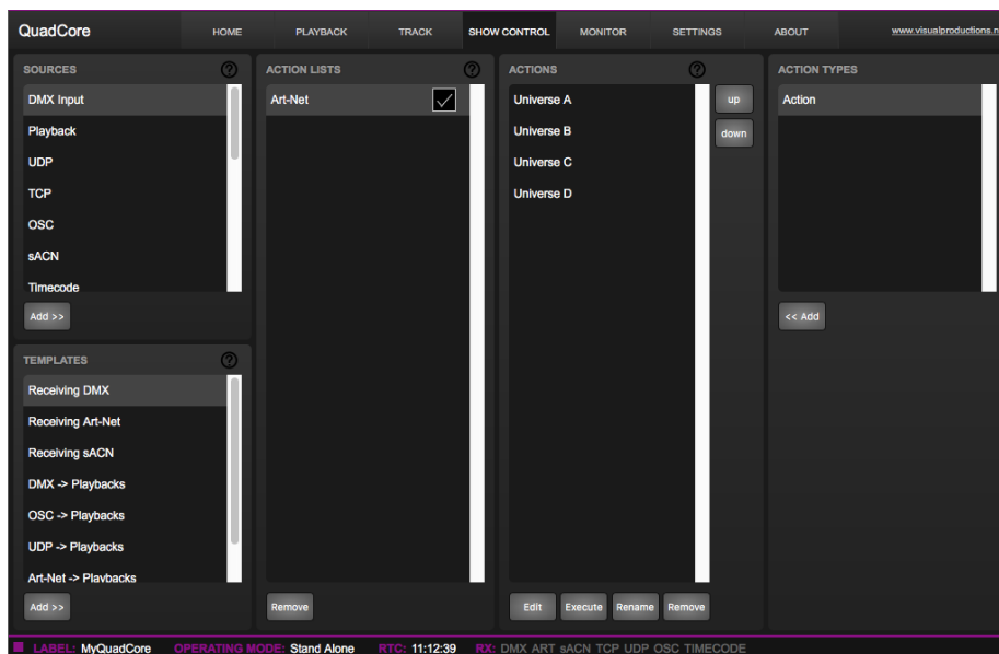
Figure 10.4: Converting Art-Net to DMX step 1
