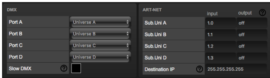
Figure 10.6: Converting Art-Net to DMX step 3
