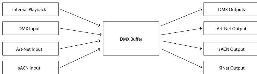
Figure 10.2: DMX merging data flow
